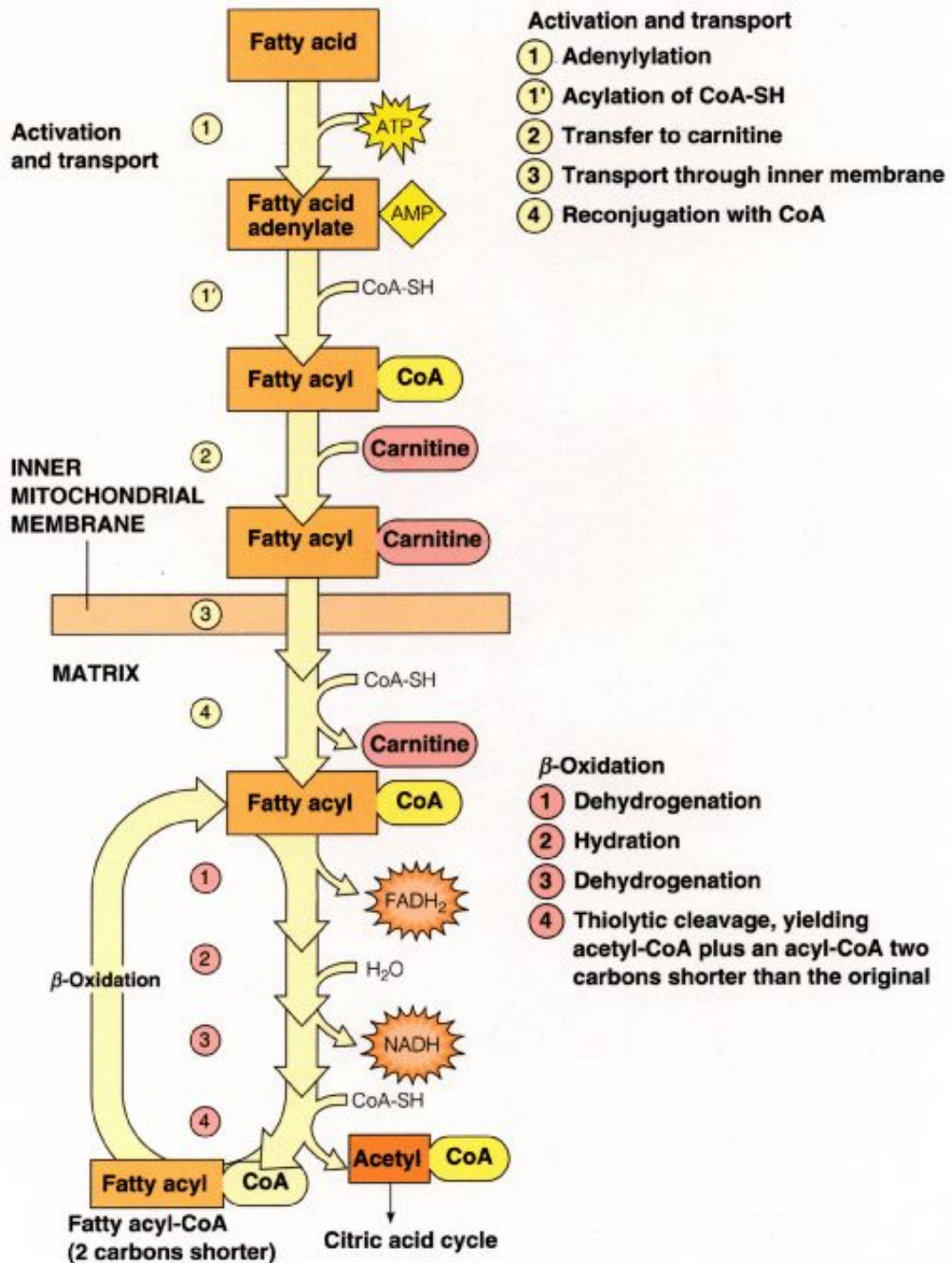
Figure 18.13 Overview of the fatty acid oxidation pathway
